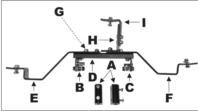
OMNI RAIL TRIO LOWER ASSEMBLY
